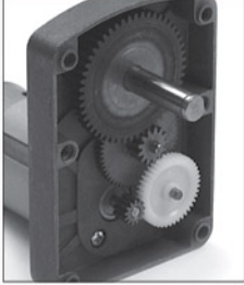
Spur Gear System
